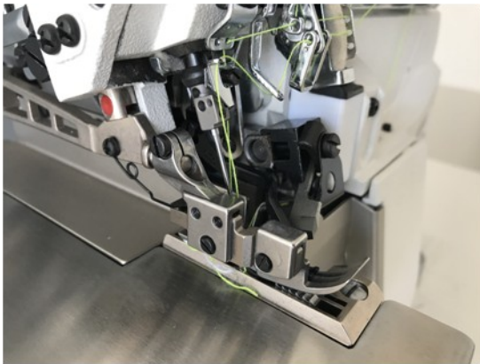
Angled knife and high needle bar stroke
