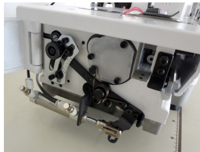
Stitch Condensing Device (CD)
