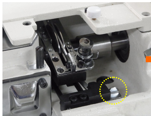
■ Slide-out thread take-up system
