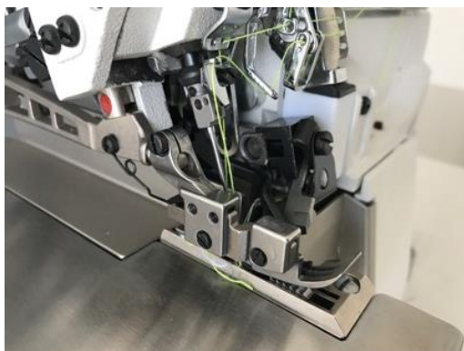
Angled knife and high needle bar stroke
