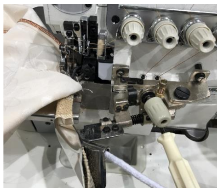
Special folder and gauge set for piping on upholstery
