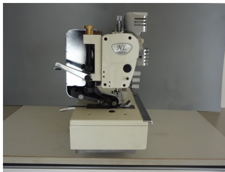
New rear puller system
